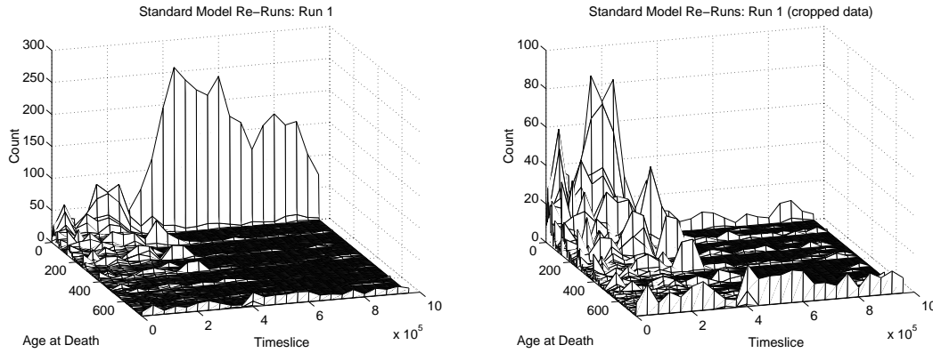
Figure 6.11: Standard Model Re-Runs: Age at Death of programs in Run 1. Left : All data. Right : Omitting data from programs that died within first 15 time slices after birth (i.e. first row of age axis). In these plots, the vertical axis (‘count’) shows the number of recorded organisms which died during that particular timeslice window that were of that particular age. The final row on the age axis show the number of programs that lived for longer than 750 timeslices.
