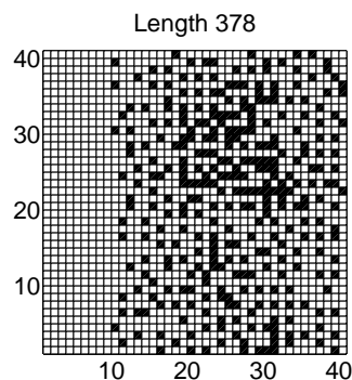
Figure 6.21: Large Energy Gradient, Run 3: Spatial Distribution of Programs at Time Slice 900,000. At this time, virtually all programs in the population were of length 378 bits.
