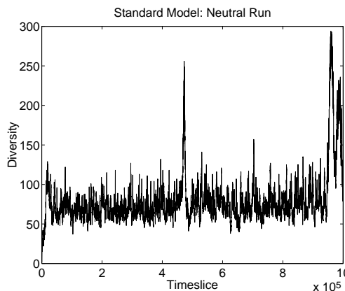
Figure 5.10: Standard Run, Neutral Shadow: Diversity.
