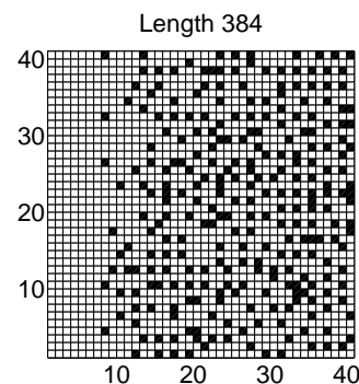
Figure 6.22: Large Energy Gradient, Run 8: Spatial Distribution of Programs at Time Slice 900,000. At this time, virtually all programs in the population were of length 384 bits.
