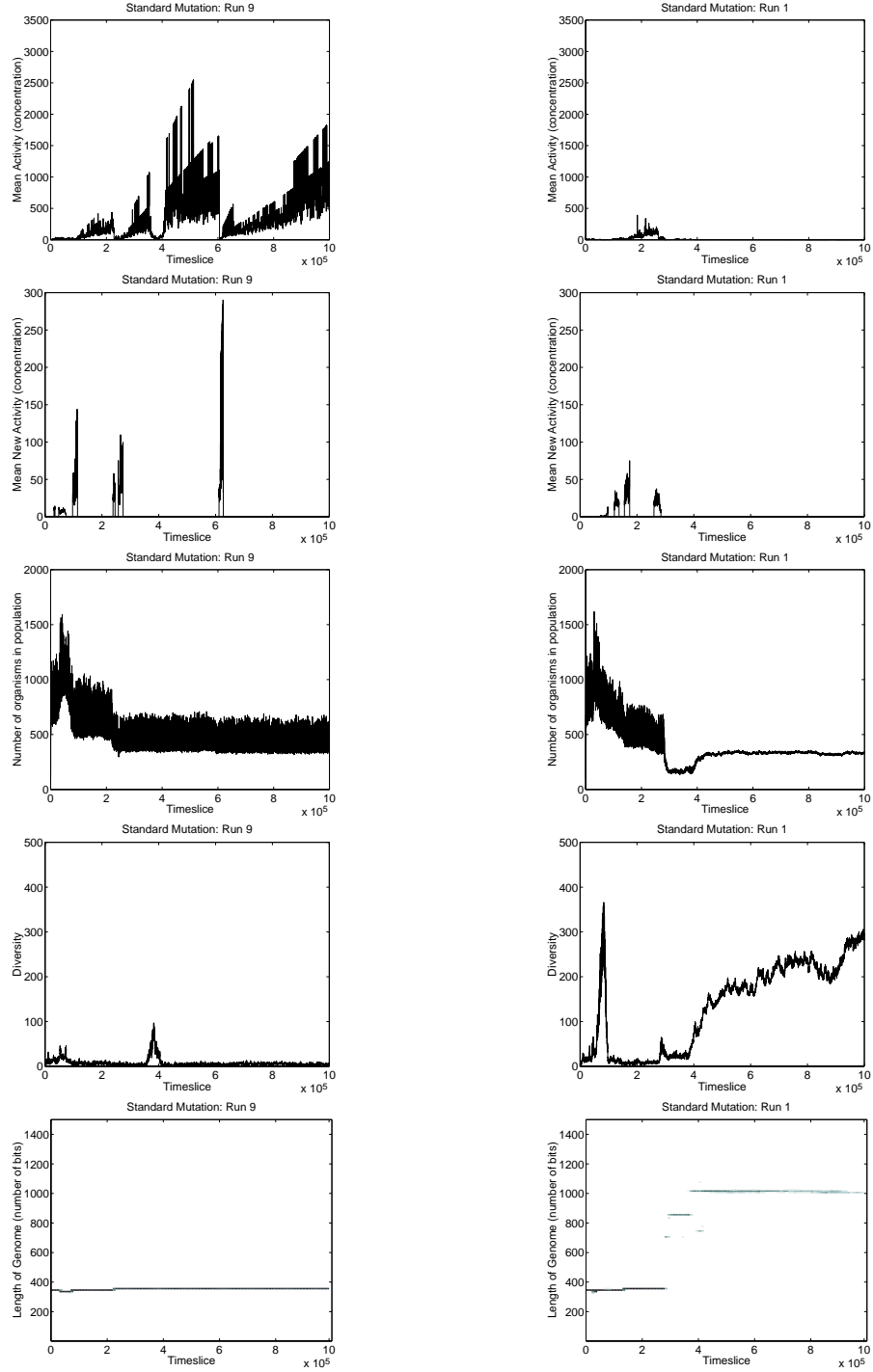
Figure 6.9: Class 2 versus Class 1 Dynamics. Left : Mean Cumulative Activity, Mean New Activity, Population Size, Diversity and Program Length for a Class 2 run (Run 9). Right : Corresponding graphs for a Class 1 run (Run 1, transition to Class 1 occurs at time slice \sim 3 \times 10^5 ).
