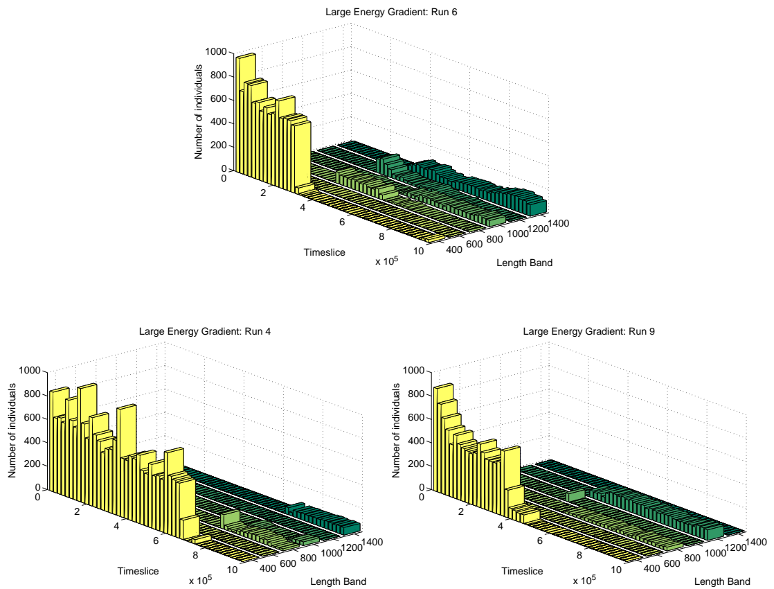
Figure 6.26: Large Energy Gradient, Runs 4, 6 and 9: Change in constitution of population over time. Each bin of the Length Band axis shows data for all programs in the population with length in a range of 200 bits, centred on the value marked. For example, the first bin, marked 400, shows the collected data of all programs of length 300–499 bits.
